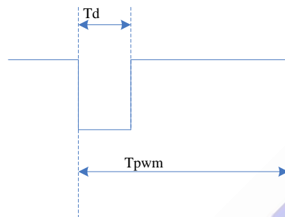
Figure 4. CPI Indication Timing
