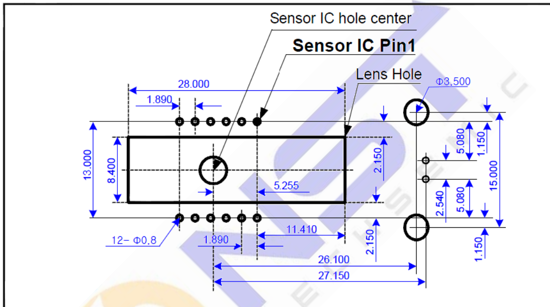
Figure 6. Recommended PCB Mechanical Drawing (Unit: mm)
