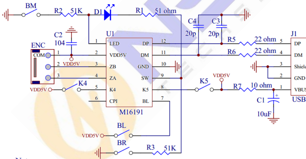
Figure 9 3D5K+ USB optical mice application.
