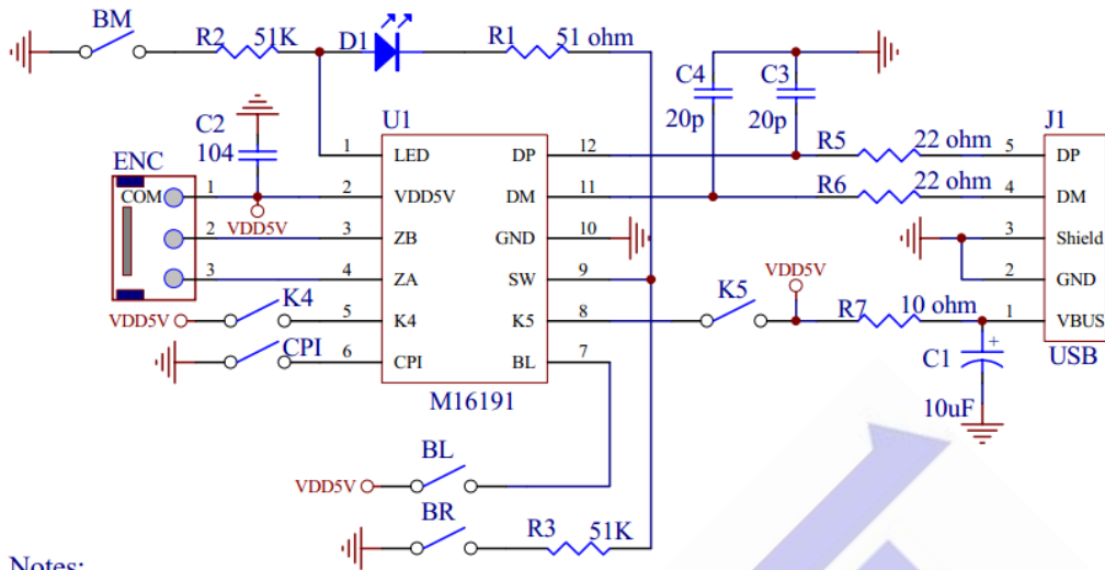
Figure 8. 3D5K++ USB optical mice application.
