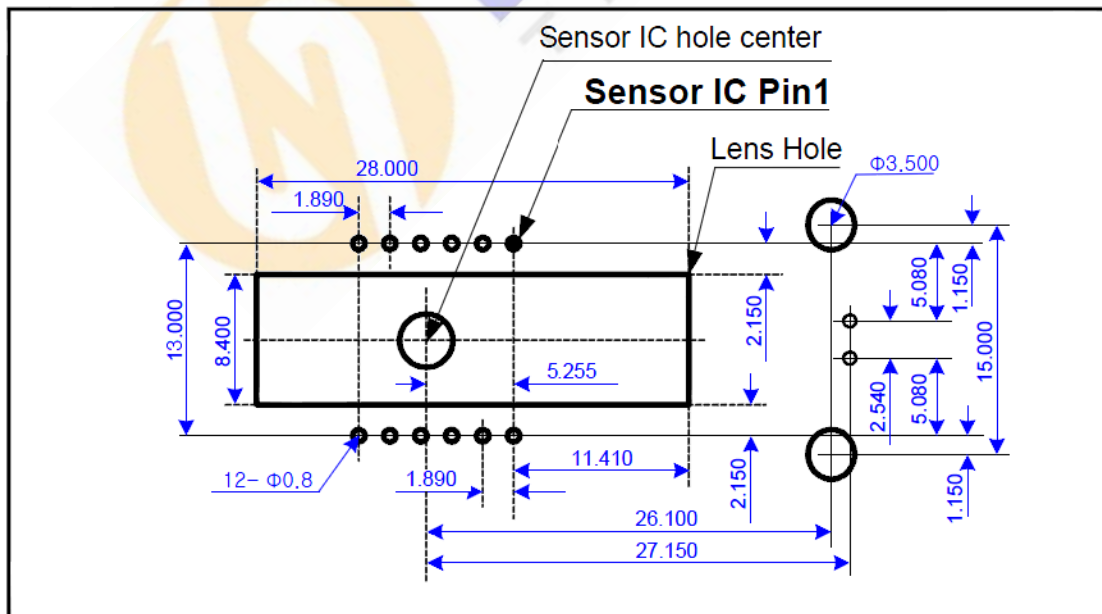
Figure 8.1 Recommended PCB Mechanical Drawing (Unit: mm)
