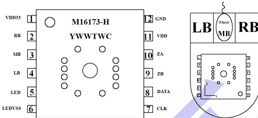
Figure 4.1 Top View Pinout
