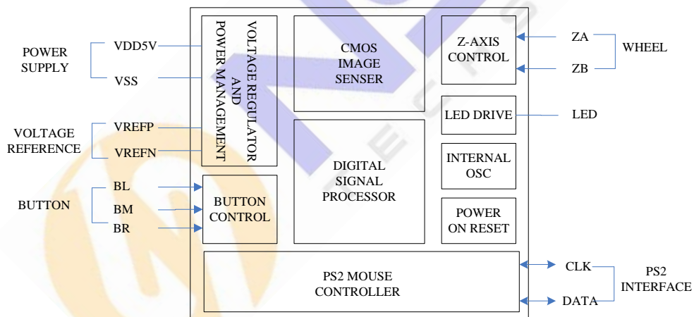
Figure 5.1 Block Diagram
