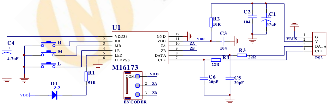
Figure 10.1 Typical 3D3K PS/2 optical mice application.
