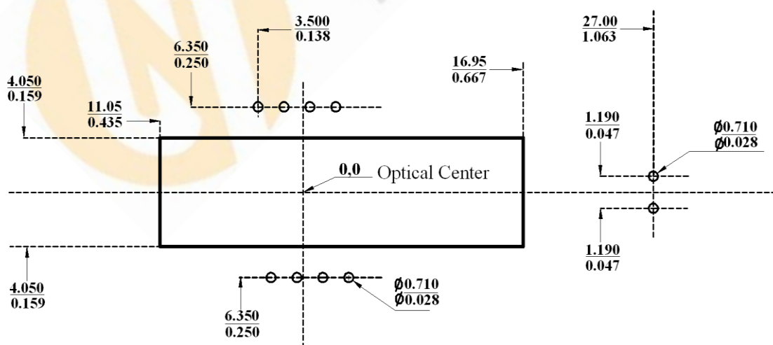
Figure 7.2 Recommended PCB Mechanical Cutouts and Spacing
