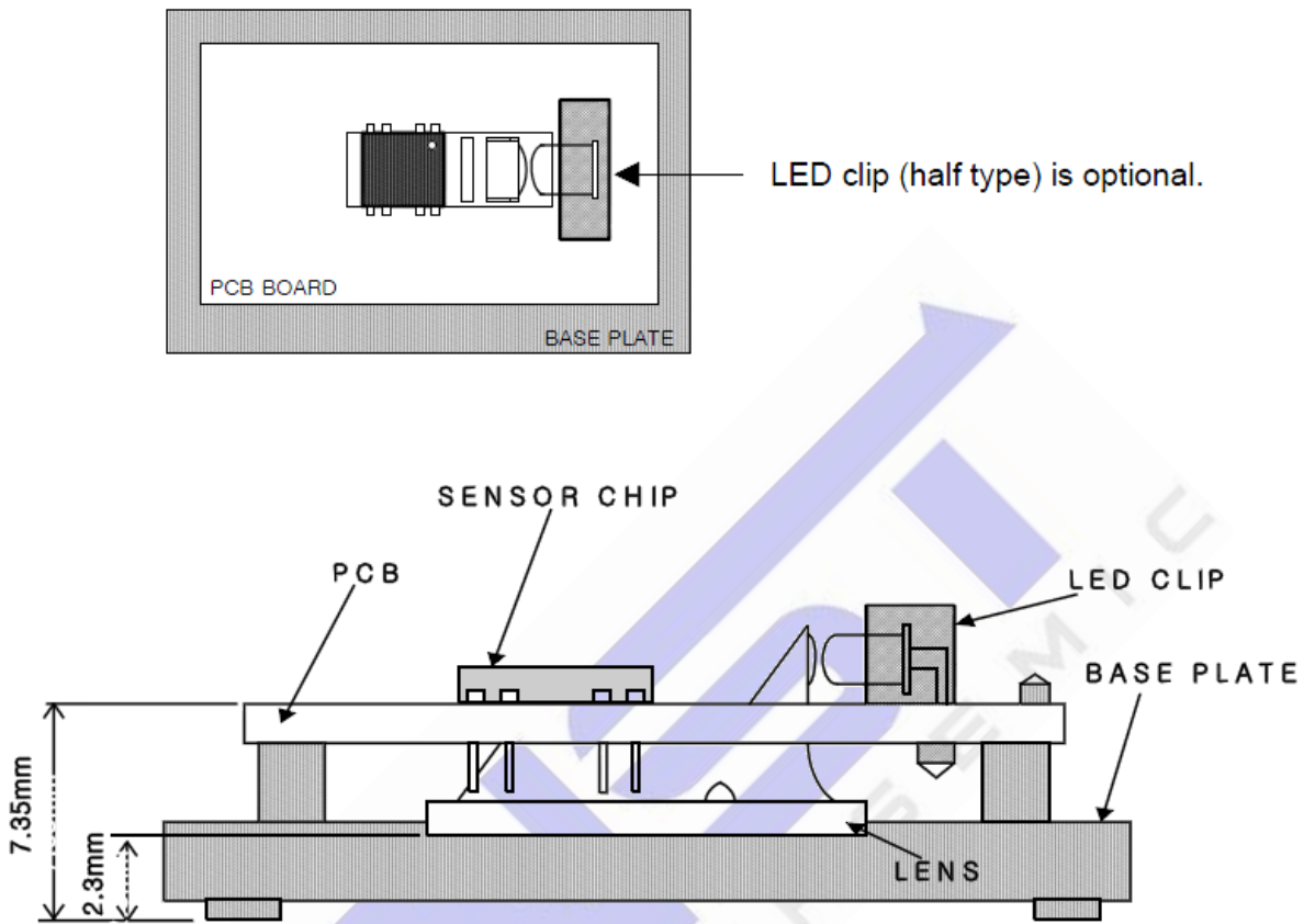
Figure 7.3 Cross Section Inside View
