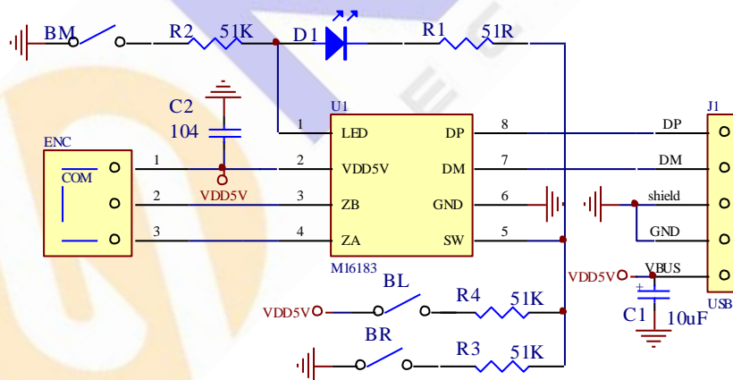
Figure 8.2 Tidy 3D3K USB optical mice application circuit
