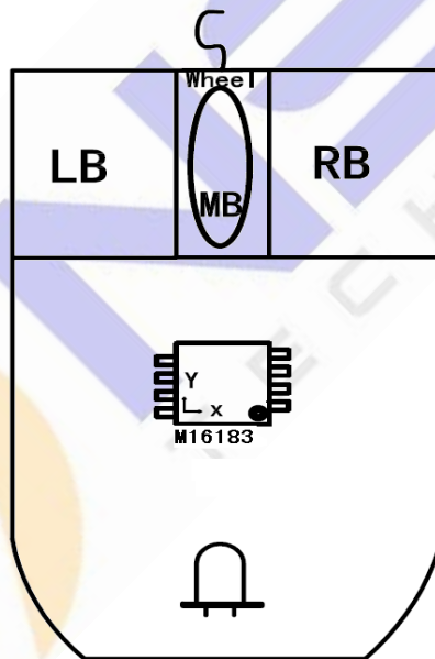
Figure 4.2 TOP View Of Mouse
