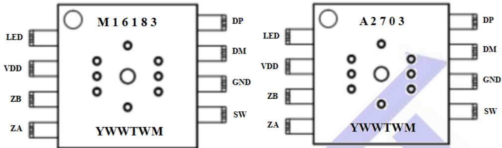
Figure 4.1 Device Pin-out
